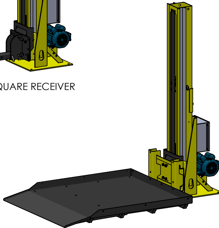
PALLET TRAY
