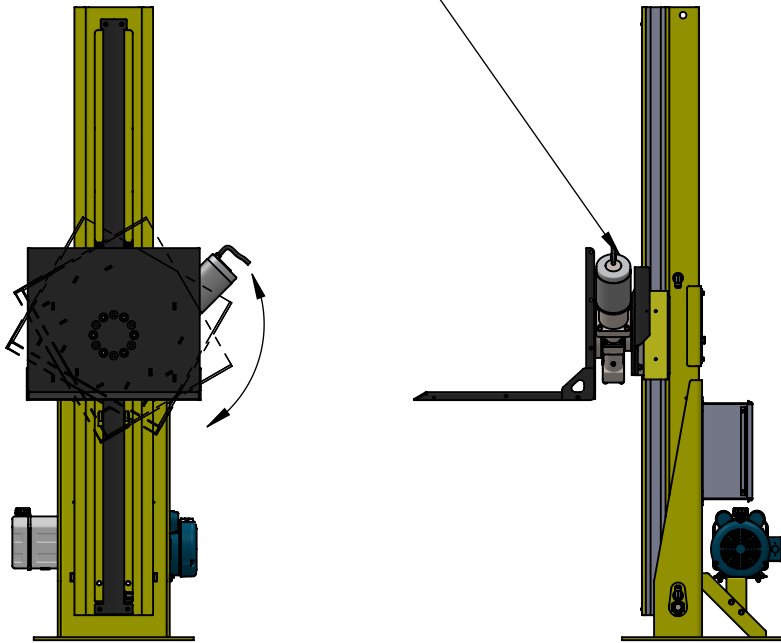
STANDARD PLATFORM WITH POWER ROTATOR
