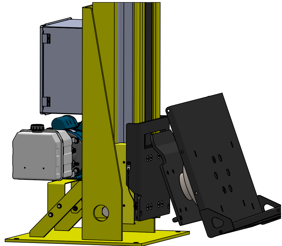
QUICK-CONNECT SYSTEM ALLOWS TOOL-FREE CHANGE OF ATTACHMENTS
