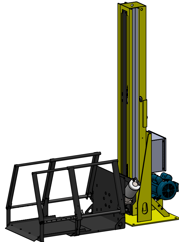
EXTENSION AND RAILS INSTALLED ON STANDARD PLATFORM
