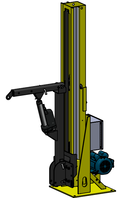
JIB ARM WITH POWERED ARM PIVOT
