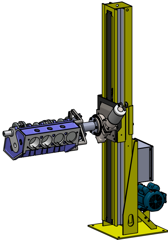
ENGINE REBUILD STATION WITH POWERED ROTATOR
